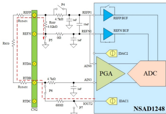
Figure 3-10 低侧基准的两线制RTD测量拓扑
