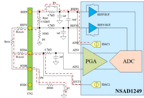
Figure 3-7 高侧基准和两个电流源的三线制RTD测量拓扑
