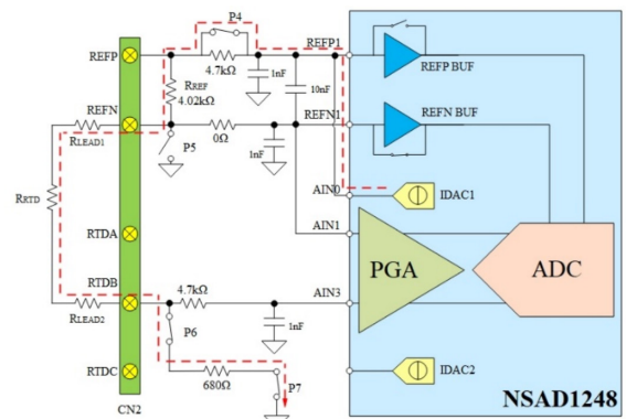
Figure 3-11 高侧基准的两线制RTD测量拓扑
